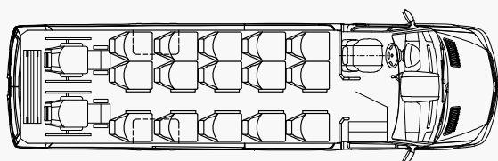
MULTILINE L FOR 15 PASSENGERS WITH 2 WHEELCHAIR PLACES
