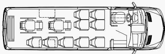
MULTILINE FOR 9 PASSENGERS WITH 2 WHEELCHAIR PLACES
