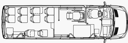
CITYLINE FOR 16 PASSENGERS WITH 2 DOORS
