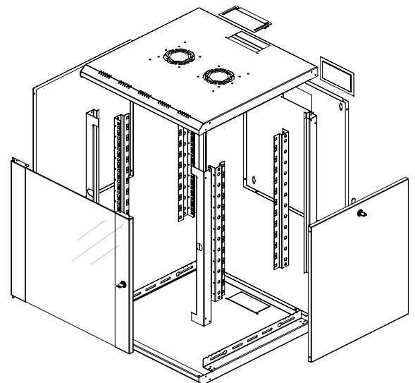
EXPLODED VIEW
