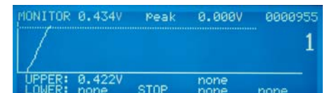
Monitor Screen – Shows weld voltage exceeding limit.
