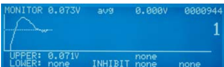
Monitor Screen – Shows 1st Pulse weld voltage exceeded limit.
