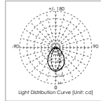
Light Distribution Curve [Unit: cd]
